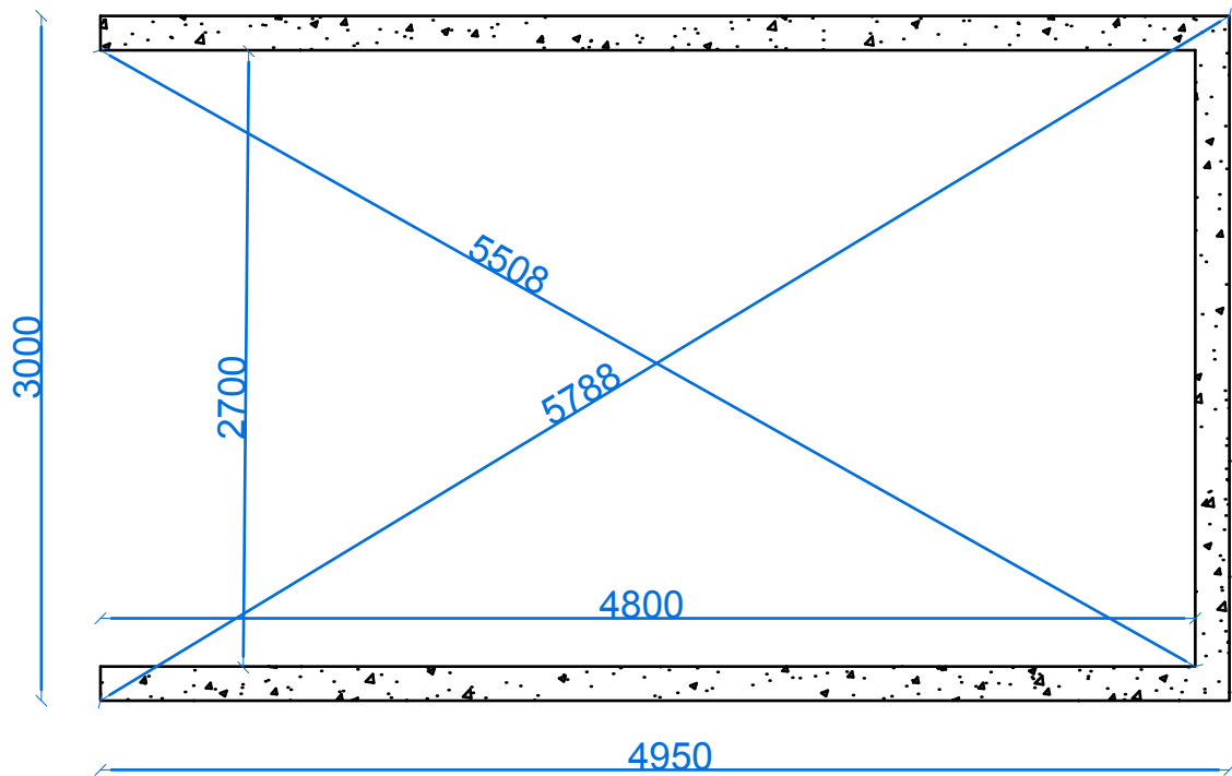
Foundation plan M 1:50
