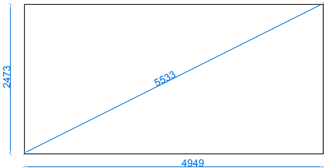
Foundation plan M 1:50
