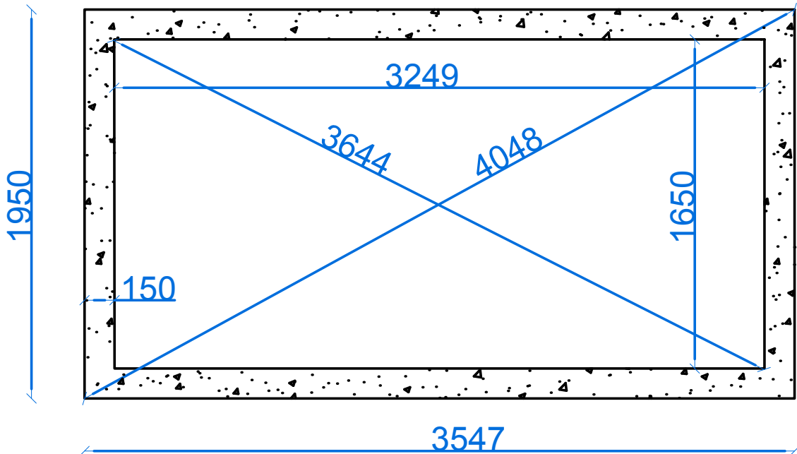
Foundation plan M 1:50
