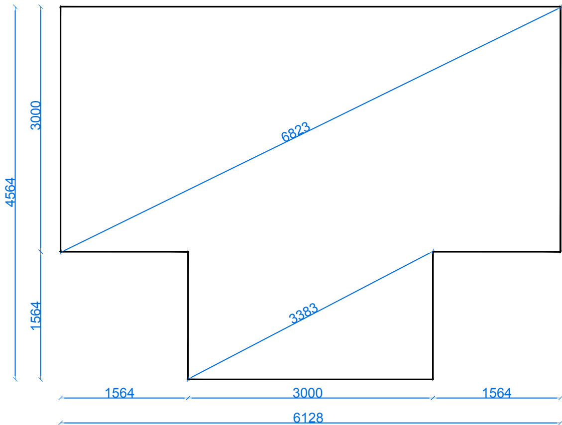
Foundation plan M 1:50
