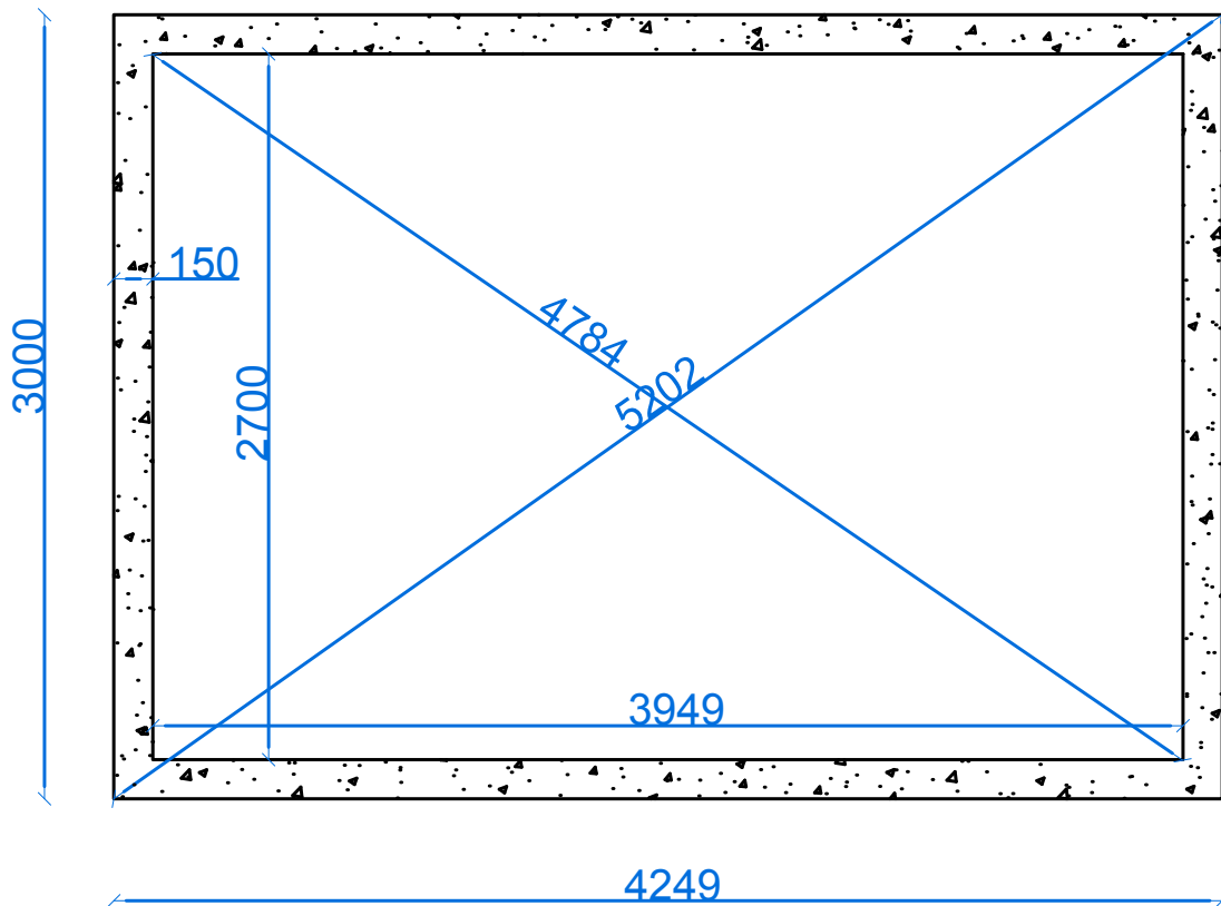
Foundation plan M 1:50
