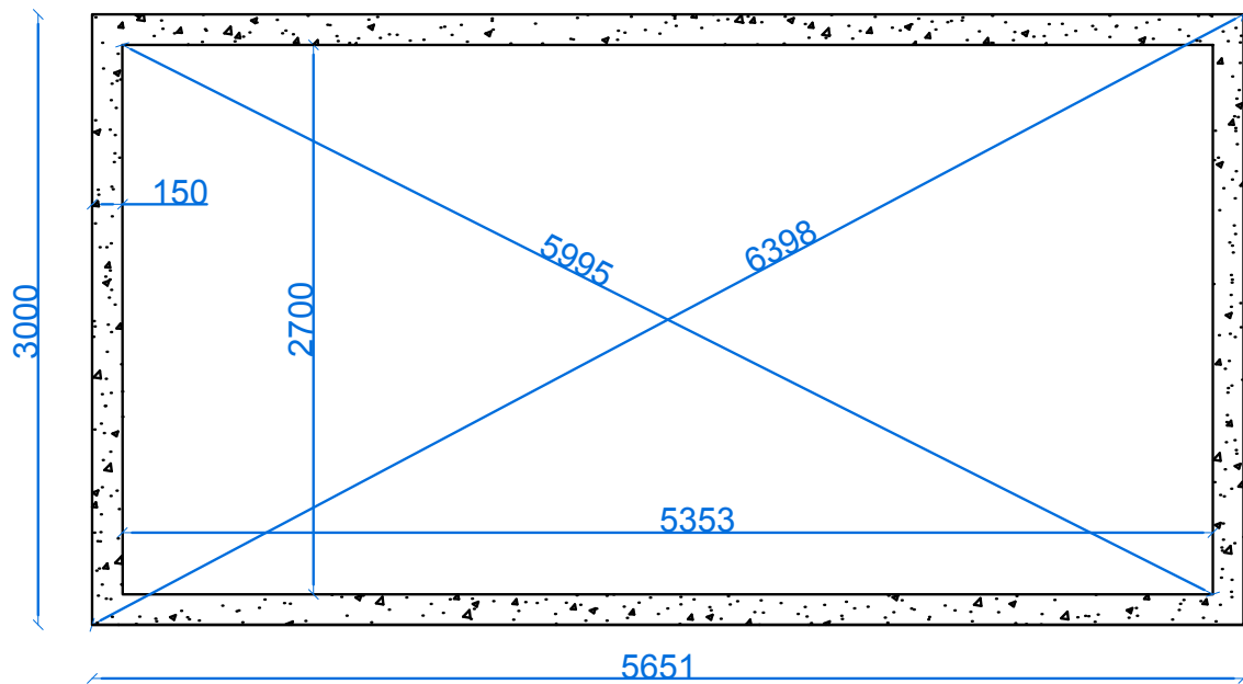
Foundation plan M 1:50
